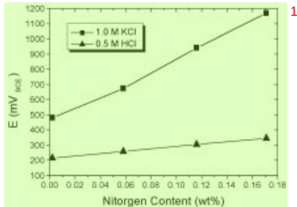
Fig. 4. Pitting potentials of type 316LN SS as a function of nitrogen content in 1 M KCl and 0.5 M HCl solutions at a scan rate of 0.2 mV/s.
