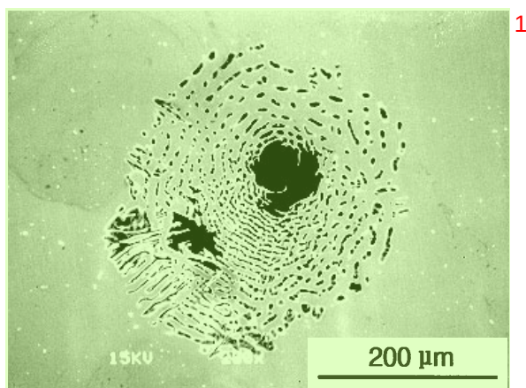
Fig. 5. Pit morphology after significant growth of a pit, taken from 20 wt.% Mn-substituted type 316LN SS with 0.314 wt.% N.
