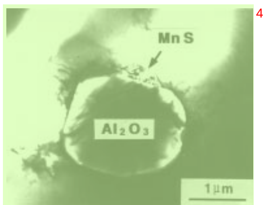
Fig. 9. TEM bright field image of MnS attached to \text{Al}_2\text{O}_3 , showing that MnS had nucleated and grown on \text{Al}_2\text{O}_3 , taken from 20 wt.% Mn-substituted type 316LN SS with 0.317 wt.% N.
