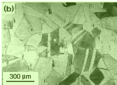
Fig. 6. Optical micrographs of (a) type 316LN SS with 0.002 wt.% N, and (b) 20 wt.% Mn-substituted type 316LN SS with 0.314 wt.% N. Chemical etching with a solution of 10% HCl + 10% HNO 3 + 15% acetic acid + 65% distilled water.
