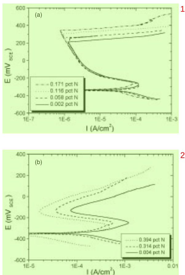
Fig. 3. Anodic polarization curves of (a) type 316LN SS and (b) 20 wt.% Mn-substituted type 316LN SS with various nitrogen contents, tested in 0.5 M HCl solution at a scan rate of 0.2 mV/s.
