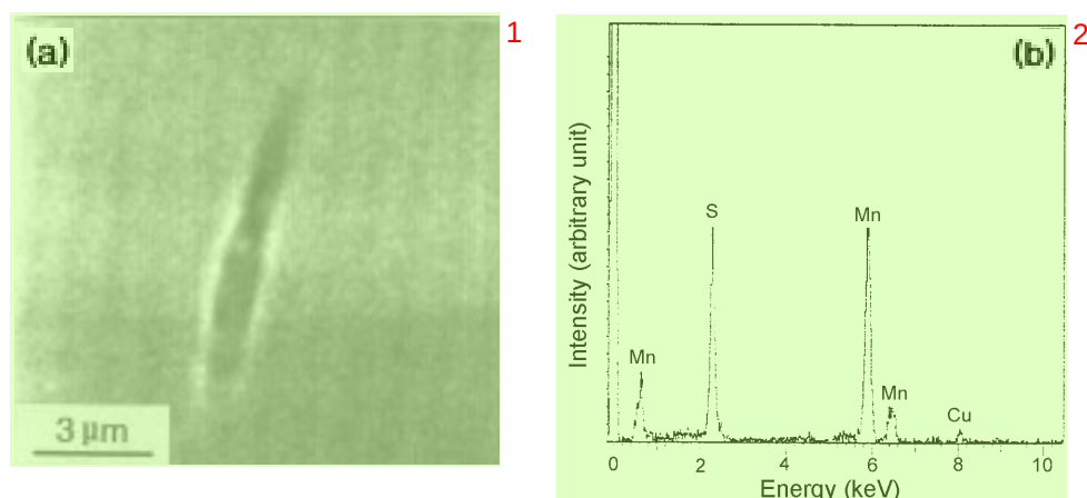
Fig. 7. (a) SEM image and (b) TEM/EDX spectrum of a sulfide inclusion, which is commonly found in 20 wt.% Mn-substituted type 316LN SS with 0.314 wt.% N.
