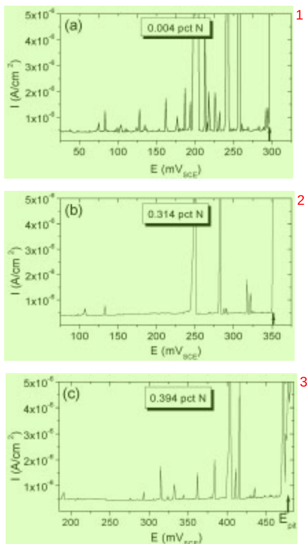
Fig. 2. Current–potential traces illustrating the occurrence of anodic current transients in the passive regions of 20 wt.% Mn-substituted type 316LN SS with nitrogen contents of (a) 0.004 wt.%, (b) 0.314 wt.% and (c) 0.394 wt.%, tested in 0.1 M KCl at a scan rate of 0.2 mV/s. The arrows in the figures are located on the pitting potentials of the alloys.
